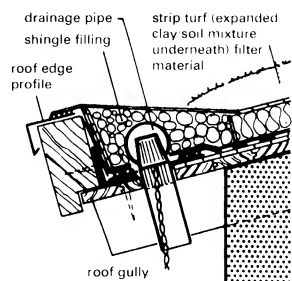
⑫ Eaves detail → ⑪
